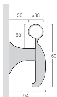
CHR1603 mounting bracket
