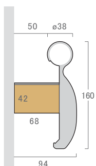
reduced ligature option available continuous timber batten with SureProtect Endure strip
