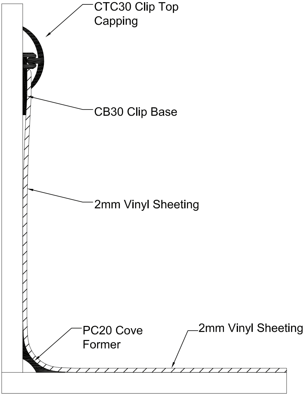
FLOORING TAKEN UP WALL USING PC20 COVE FORMER AND CB CLIP TOP CAPPING AND BASE
